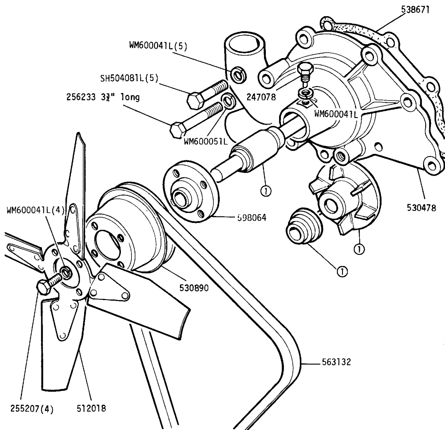
Water pump assembly ERC9178 ① Water pump overhaul kit RTC3072
